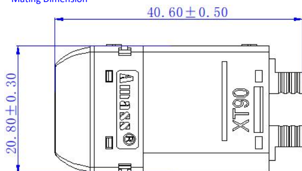
Mating Dimension
