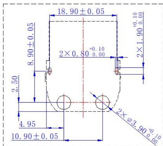
Mating Dimension
