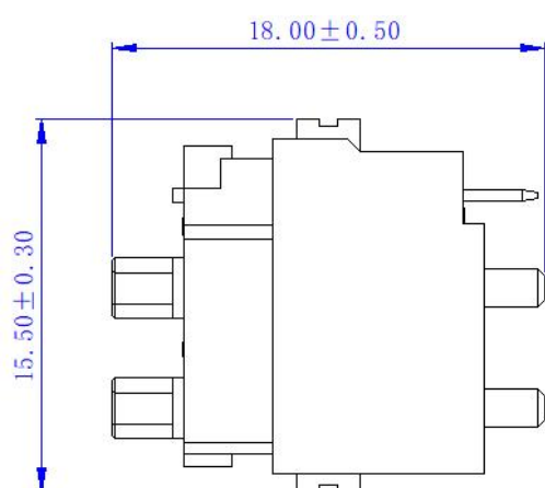
Mating Dimension
