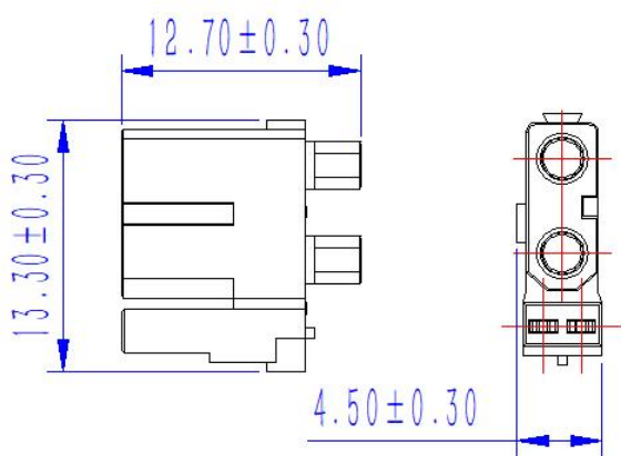
Stacking Dimension
