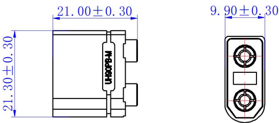
Stacking Dimension
