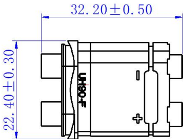
Mating Dimension
