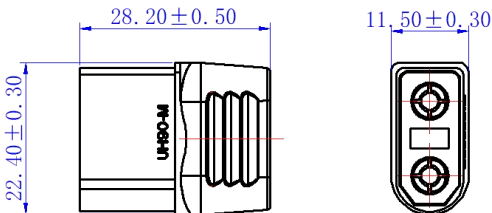
Mating Dimension
