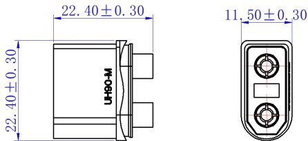
Stacking Dimension
