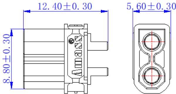
堆叠尺寸 Outline drawing size
