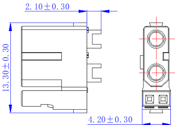
堆叠尺寸 Outline drawing size
