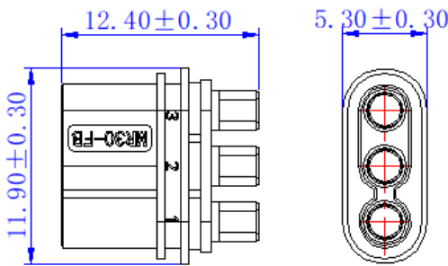
带后盖堆叠尺寸 Outline drawing size with back cover
