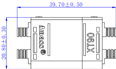
带后盖互配尺寸 Matching size with back cover
