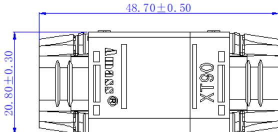
带后盖互配尺寸 Matching size with back cover
