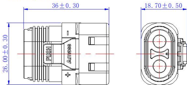
Stacking Dimension
