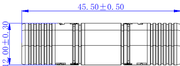
带后盖互配尺寸 Matching size with back cover
