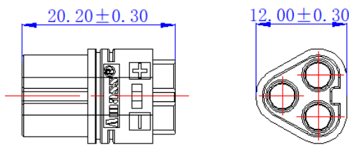
带后盖堆叠尺寸 Outline drawing size with back cover
