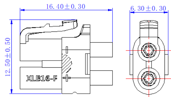
带后盖堆叠尺寸 Outline drawing size with back cover
