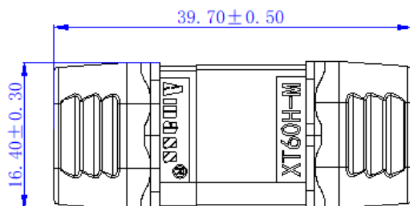
带后盖互配尺寸 Matching size with back cover
