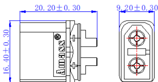
带后盖堆叠尺寸 Outline drawing size with back cover
